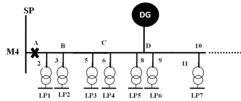
Figure 5 DG unit connected at D of main feeder M4 of the test system
