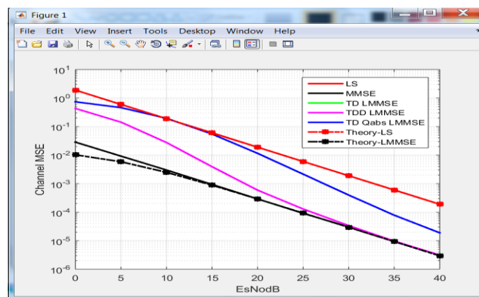
Figure: 4.1 Channel MSE and E/N Plot.
