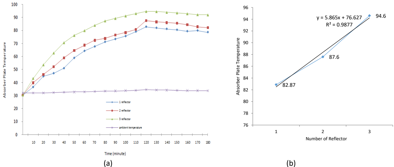
Figure 4. The (a) temperature of the absorber plate of the solar box heater as influenced by the different number of reflectors for 180 minutes of observation and (b) the relationship between the number of reflectors and the temperature of the heat absorber plate.
