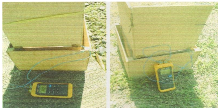
Temperature measurement at various parts of the solar box heater using digital thermometer
