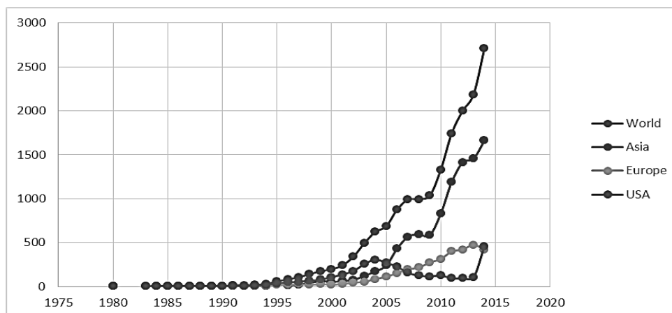
Fig. 4. The dynamics of the number of patents in micro- and nano-technologies for the world, Asia, Europe, and the USA in 1980–2014
