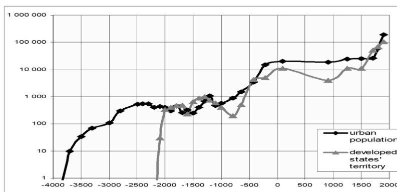
Fig. 3. Dynamics of World Urban Population (thousands) and the Size of the Territory Controlled by the Developed and Mature States and Their Analogues (thousands km 2 ), till 1900 CE, logarithmic scale
