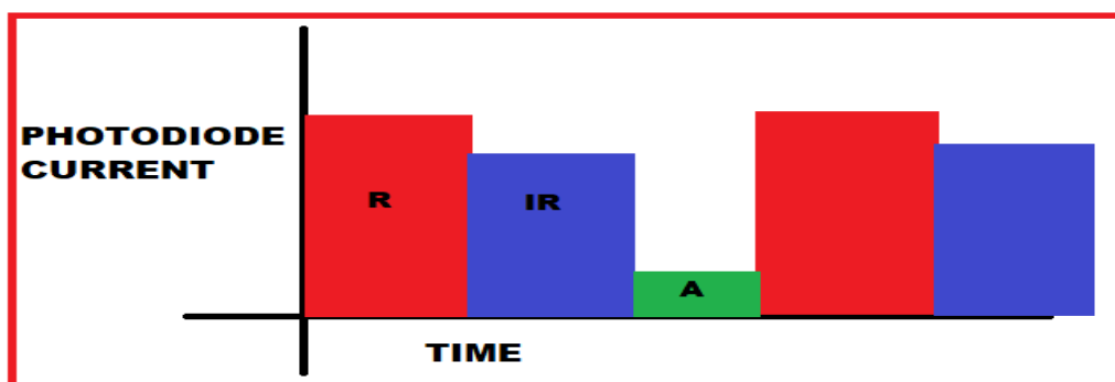
Figure 3. Pulsation of the arterial blood
