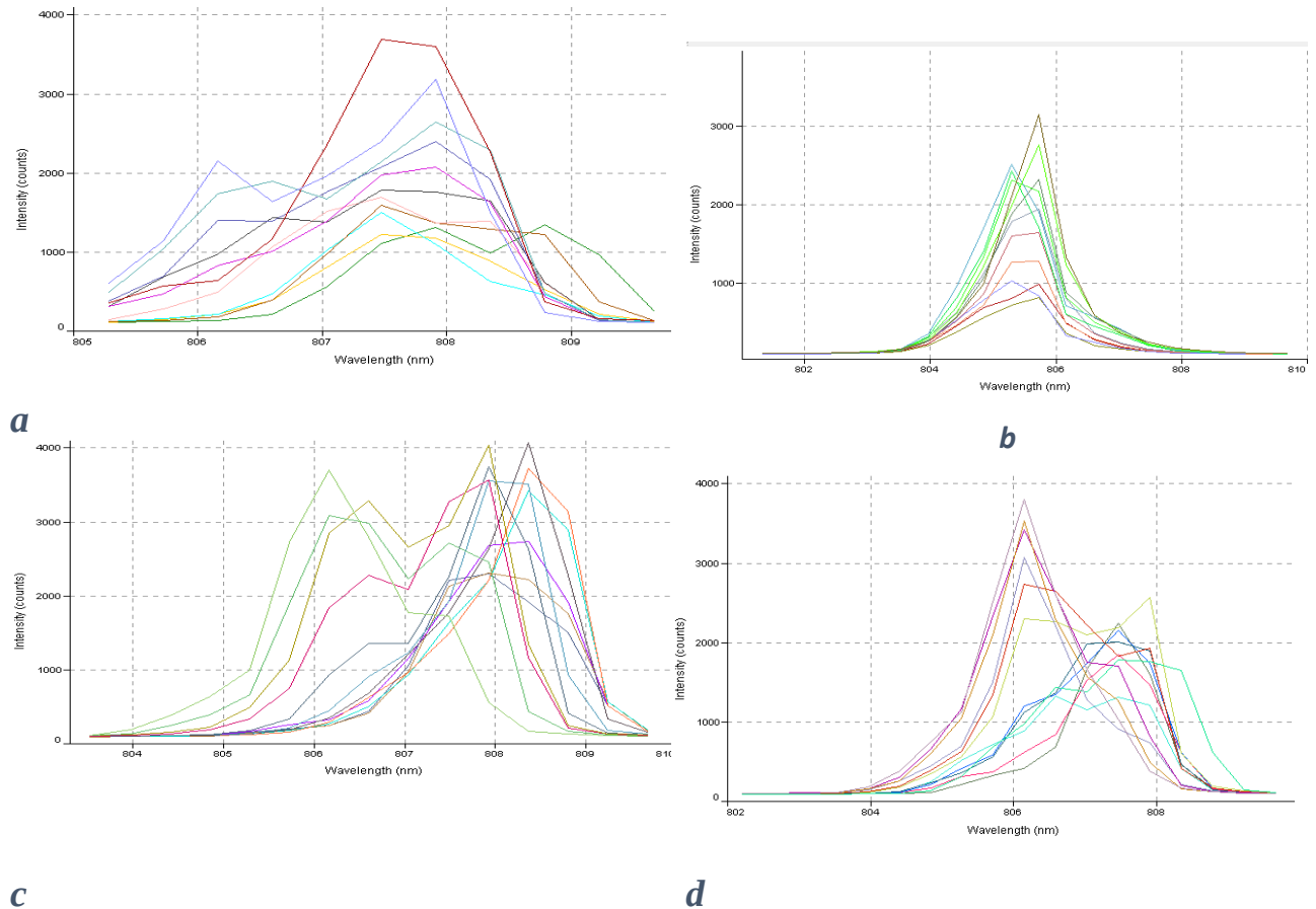
Figure 4: Transmission spectra of 2cm LMA-10 PCF interferometer for sensing leak at different temperature for polymer pipe S1 a-(26), b-(36), c-(40), d-(50)
