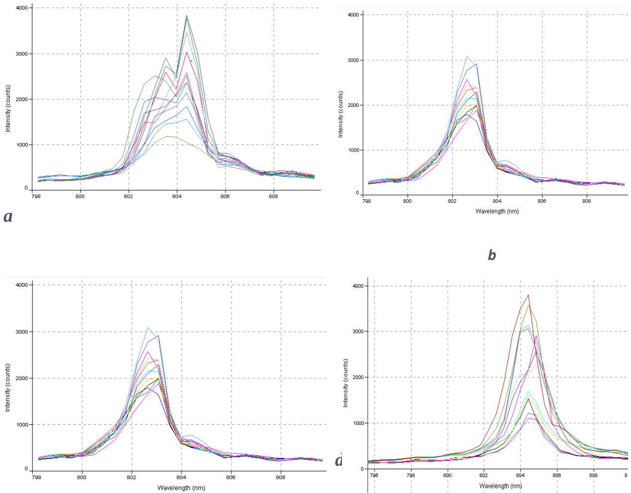
Figure 8: Transmission spectra of 2.5 cm LMA-10 PCF interferometer for sensing leak at different temperature for Polymer pipe S2 a-(26), b-(36), c-(40), d-(50)
