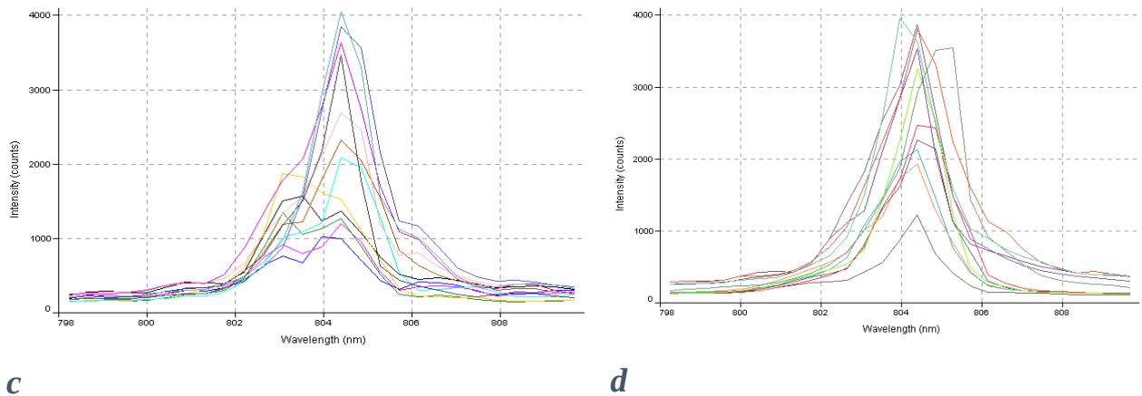
Figure 6: Transmission spectra of 2.5 cm LMA-10 PCF interferometer for sensing leak at different temperature for metal pipe S2 a-(26), b-(36), c-(40), d-(50)
