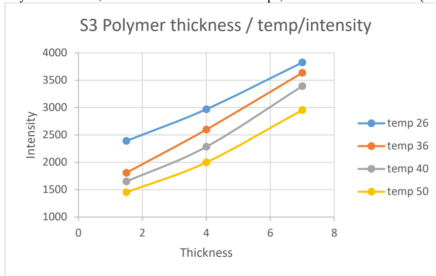
Figure 13: The relationship between intensity and (t1.t6.t12) wall thickness for different temperature of 3 cm LMA-10 PCF sensor of polymer pipe S3 (sensitivity = 0.14 nm/RIU)
