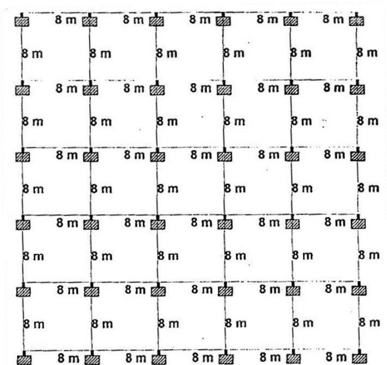
Figure 1 Plan of the Building
