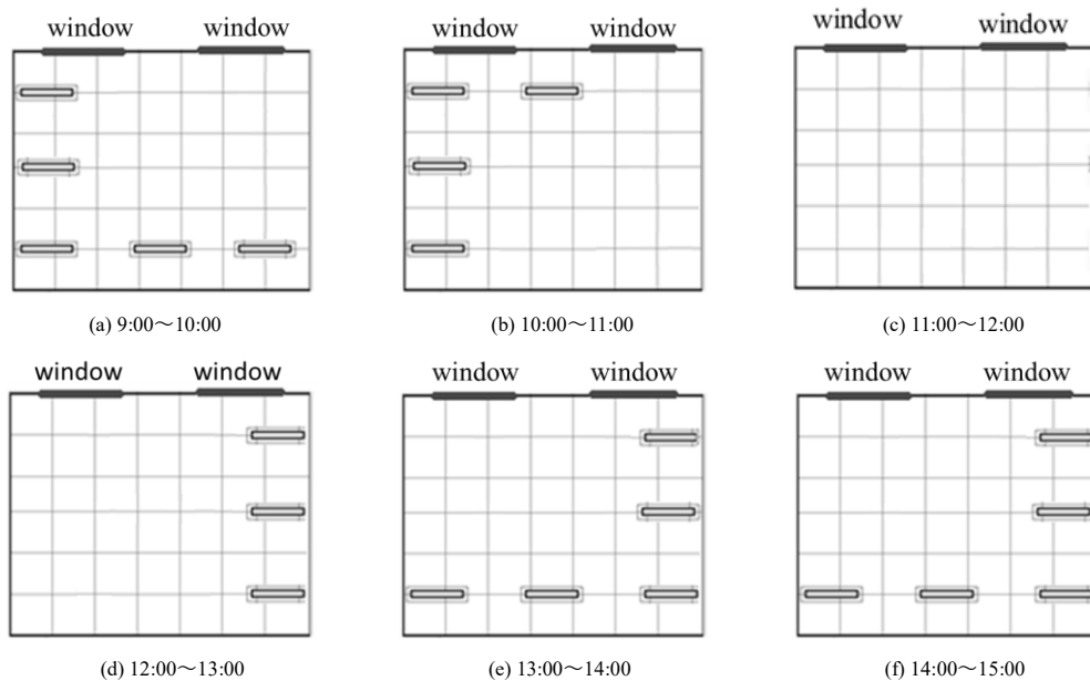
Fig. 13. Lighting fixture placement pattern for spring and autumn
