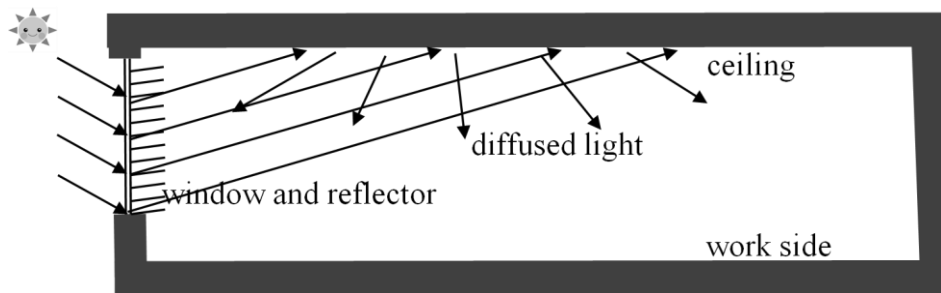
Fig. 2. Daylighting method by reflectors
