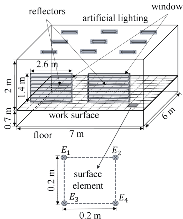
Fig. 1. Model diagram for the simulation
