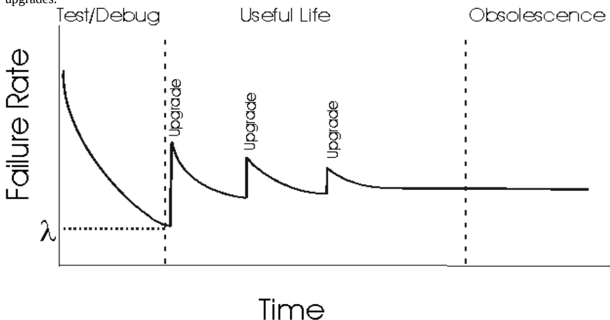
Figure 2. Revised bathtub curve for software reliability
