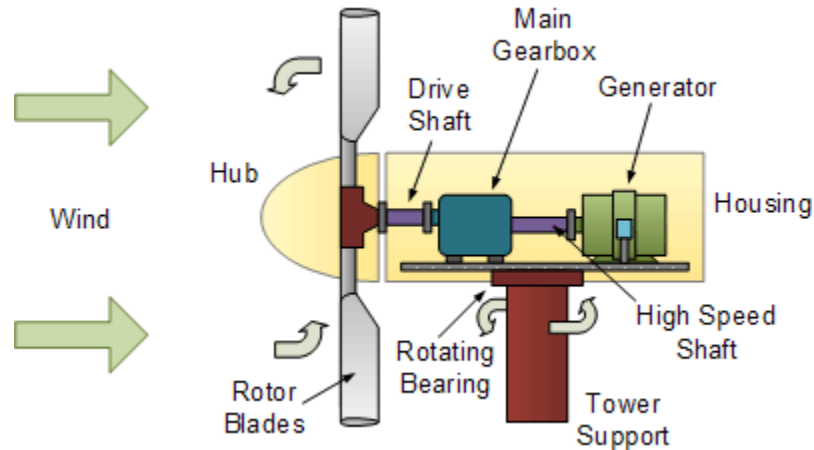
Fig. (1) Typical Wind Turbine Generator Design
