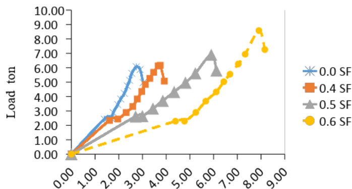
Figure (9) Load deflection for different % steel fiber (concrete f_{cu,30} MPa)
