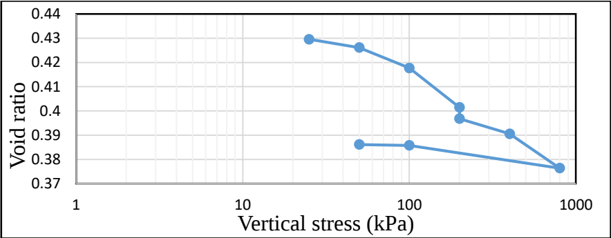
Fig.6: Variation of void ratio with vertical stress for GA soil prepared at w=14\% , \gamma_{dry}=18.10\text{ kN/m}^3 in single oedometer test.
