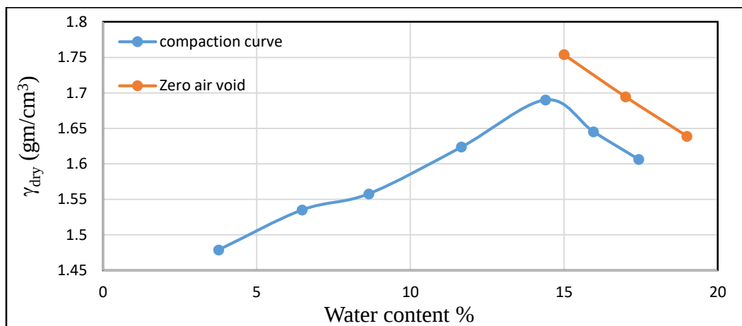
Figure 3: Compaction curve for Tikrit soil (□=55%).
