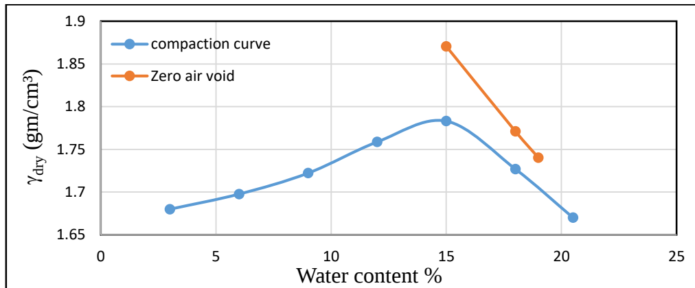
Figure 1: Compaction curve for Arar soil (□=12%).
