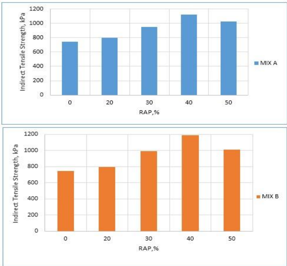
Fig.4. Indirect tensile strength for conditioned for Mix A, Mix B
