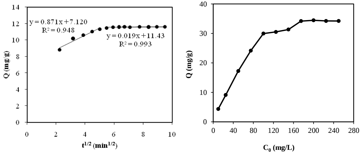
Figure 8: Linear plot of intra-particle diffusion model for the adsorption of MB dye on corn cobs
