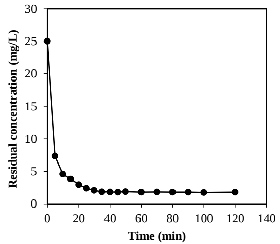
Figure 6: Residual concentration of MB as a function of time ( C_0 = 25 mg/L; Adsorbent = 0.2 g; V = 100 mL; pH = 6.4; 500 rpm; T = 25 \pm 2^\circ\text{C} )
