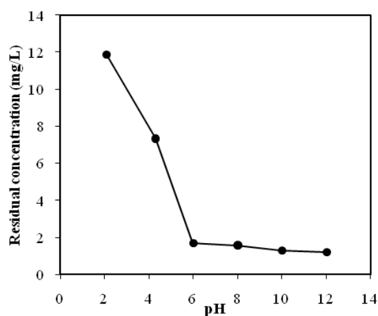
Figure 4: Residual concentration of MB as a function of pH ( C_0 = 25 mg /L; Adsorbent = 0.2 g; V = 100 mL; Contact time = 2 h; 500 rpm; T = 25 \pm 2^\circ\text{C} )
