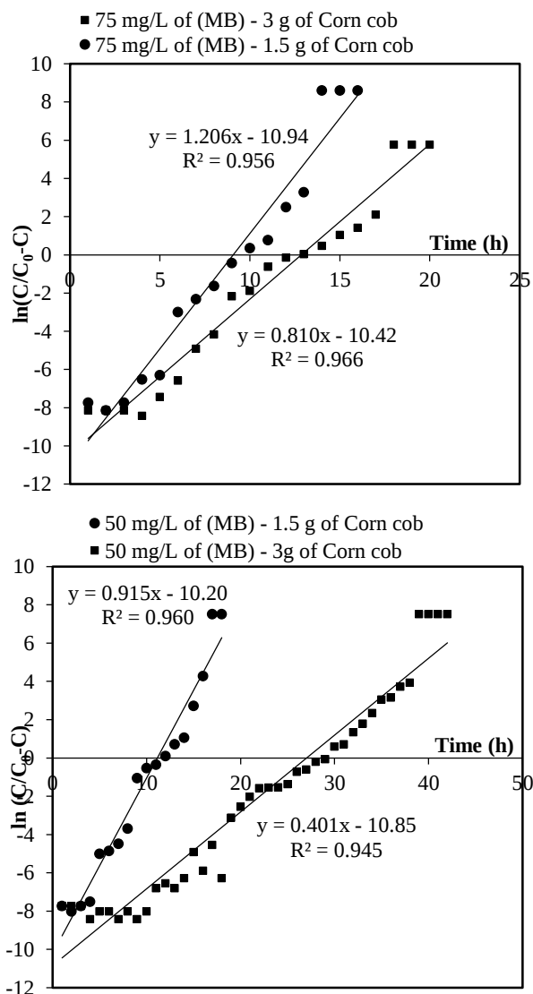
Figure 14: Linearized form of Yoon-Nelson model for the adsorption of MB dye on corn cobs bed ( C_0 = 50 and 75 mg/L; bed weight = 1.5 and 3 g; pH = 6.4 ; T = 25 \pm 2^\circ C )
