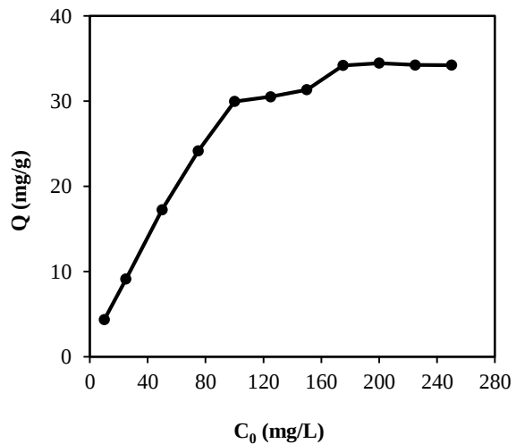
Figure 9: Effect of the initial concentration of MB dye on the discoloration ( V = 100 mL; Adsorbent = 0.2 g; pH = 6.4; Contact time = 2 h; 500 rpm; T = 24 \pm 2^\circ\text{C} )
