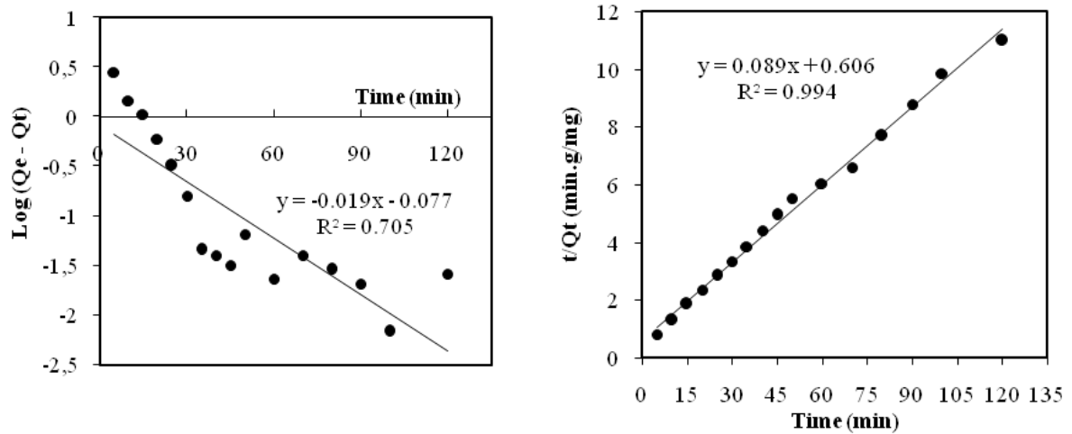
Figure 7: Pseudo-first-order and pseudo-second-order kinetic plots for MB adsorption onto corn cobs ( C_0 = 25 mg/L; Adsorbent = 0.2 g; V = 100 mL; pH = 6.4; 500 rpm; T = 25 \pm 2^\circ\text{C} )
