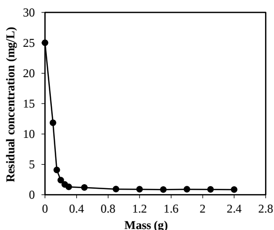
Figure 3: Residual concentration of MB as a function of corn cobs weight ( C_0 = 25 mg/L; pH=6.4; 500 rpm; Contact time = 2h; V=100 mL; T = 25 \pm 2^\circ\text{C} )
