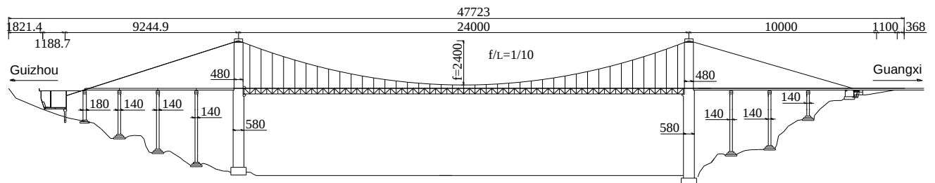
Fig.1 Layout drawing of the bridge before reinforcement
