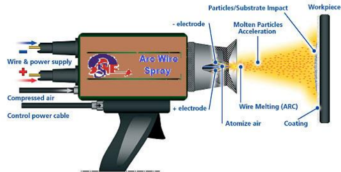
Fig. 8 (c) Schematic view of electric arc wire spray process gun
