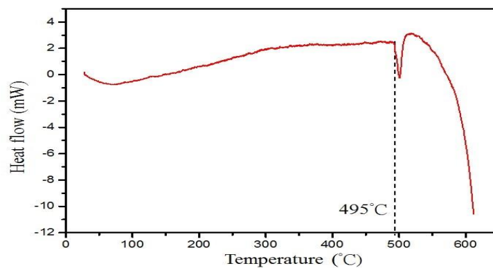
Fig. 4 DSC curve of as-received 2024 Al alloy (F).
