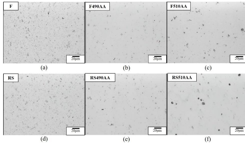
Fig. 8 Microstructures without etching for eutectic phase observation (ED plane) of (a) F, (b) F490AA, (c) F510AA (d) RS, (e) RS490AA, and (f) RS510AA.
