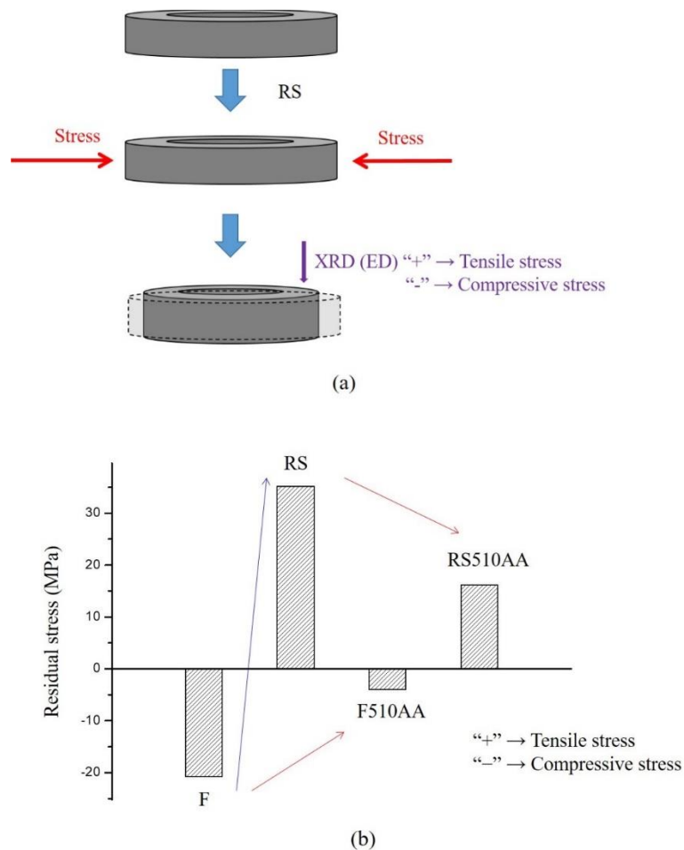
Fig. 15 (a) Illustration of residual tensile stress and compressive stress and (b) residual stress.
