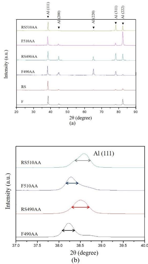
Fig. 16 XRD patterns of materials: (a) from 20° to 90° and (b) around (111) peak.
