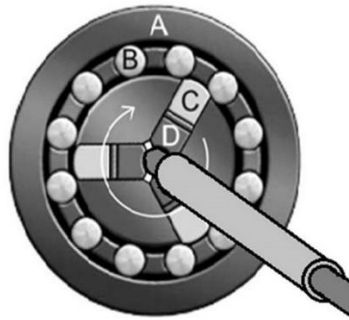
Fig. 1 Illustration of rotary swaging equipment.
