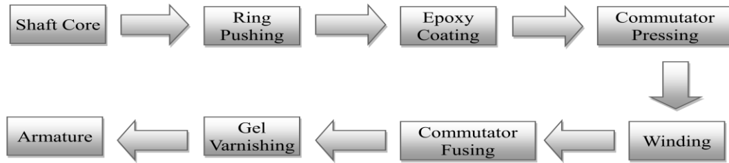
Figure 3: Process Flow
