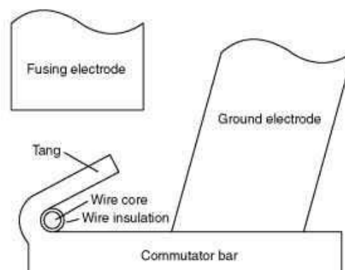
Figure 2: Commutator Fusing Process
