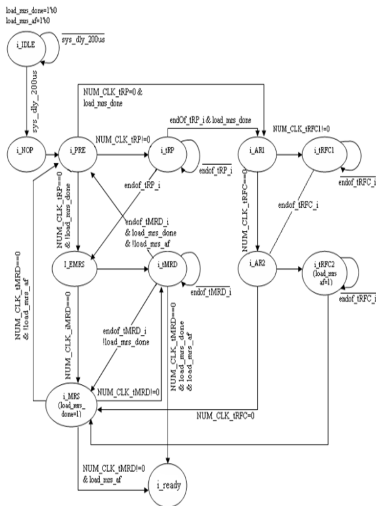
Figure 4: Initial FSM State Diagram
