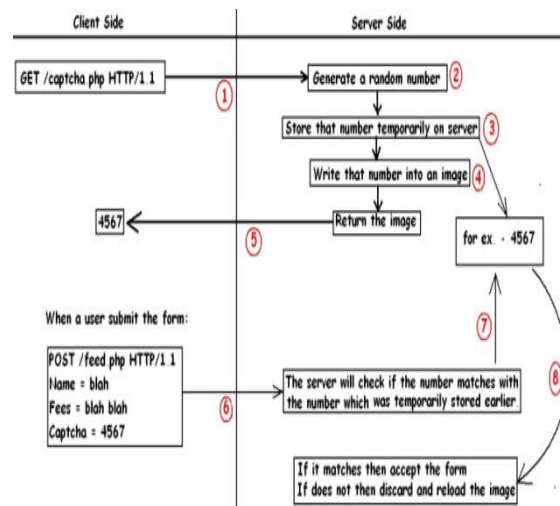
Figure 1 Working of CAPTCHA [5]
