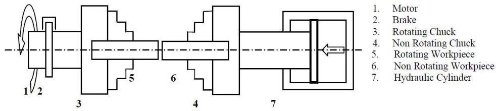
Figure 1: Layout of Continuous Drive Friction Welding [1]
