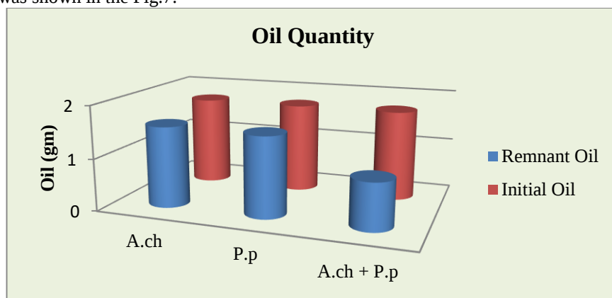
Fig 7: Comparative graph of oil degradation by A.ch, P.p and A.ch + P.p in 1% oil before optimization.
