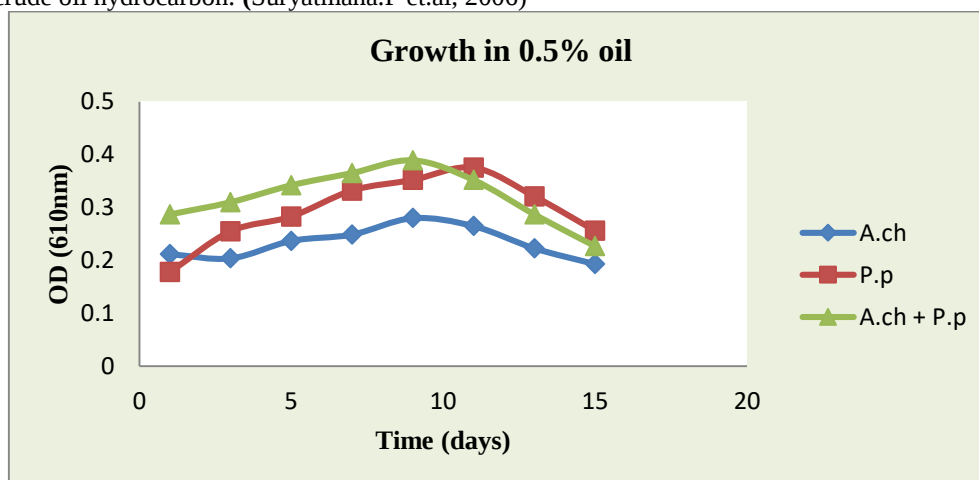
Fig 1: Comparative graph of growth of A.ch, P.p and A.ch + P.p in 0.5% oil.
