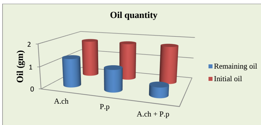
Fig 8: Comparative representation of difference of oil quantity before and after optimization.
