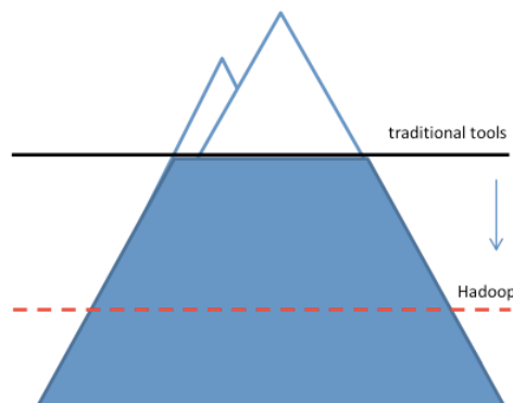
Fig 1: Hadoop Level
