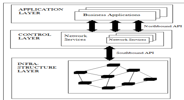
Fig. 1. SDN Architecture
