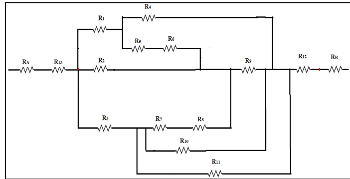
Fig. 11 Resistance circuit of plastic coated filler mullion
