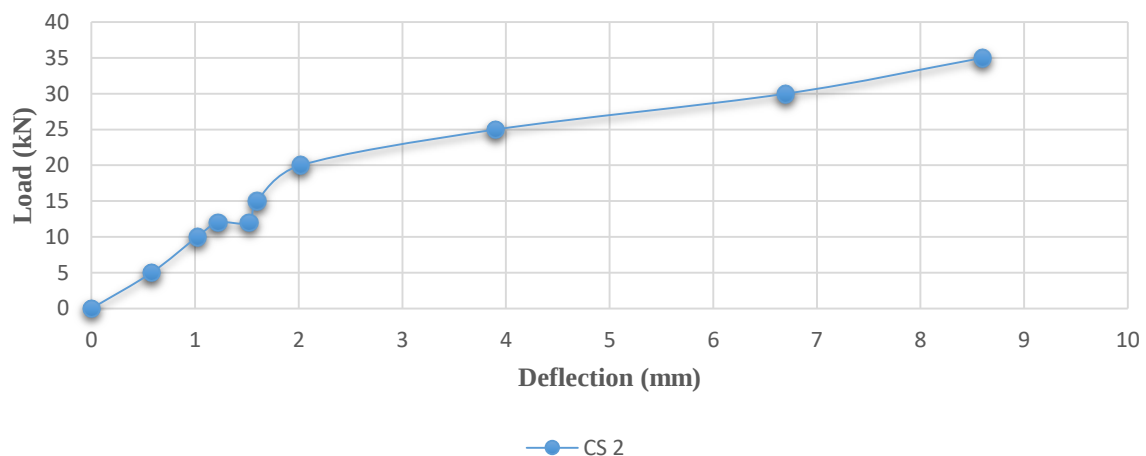
Chart 4. Load vs Deflection curve for composite slab 2
