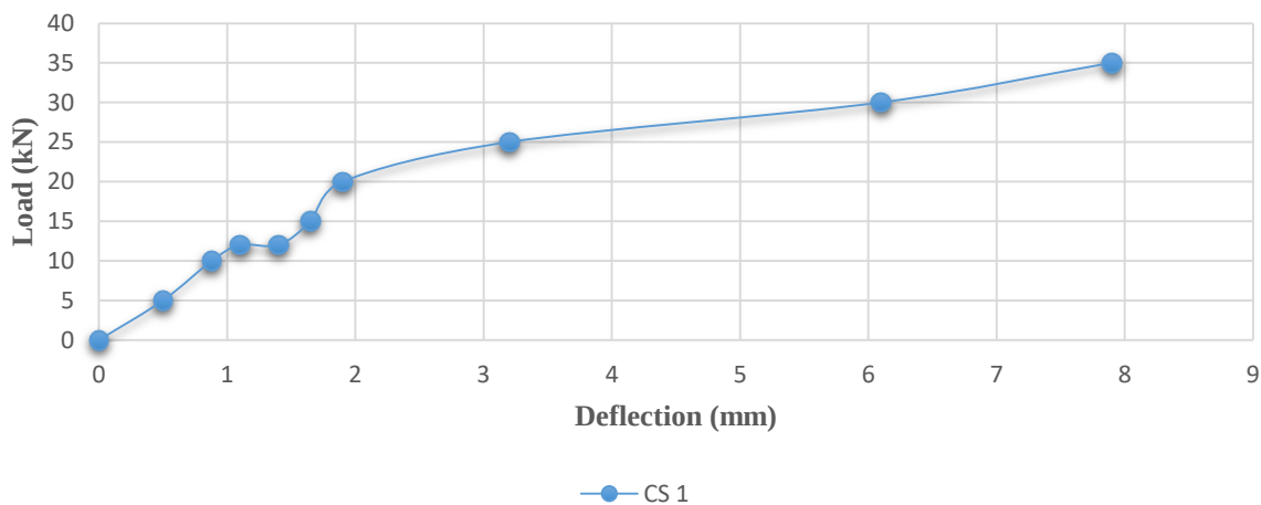
Chart 3. Load vs Deflection curve for composite slab 1
