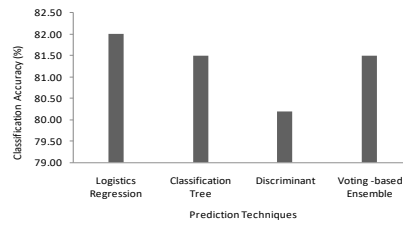
Fig 4: Classification Accuracy for Test dataset
