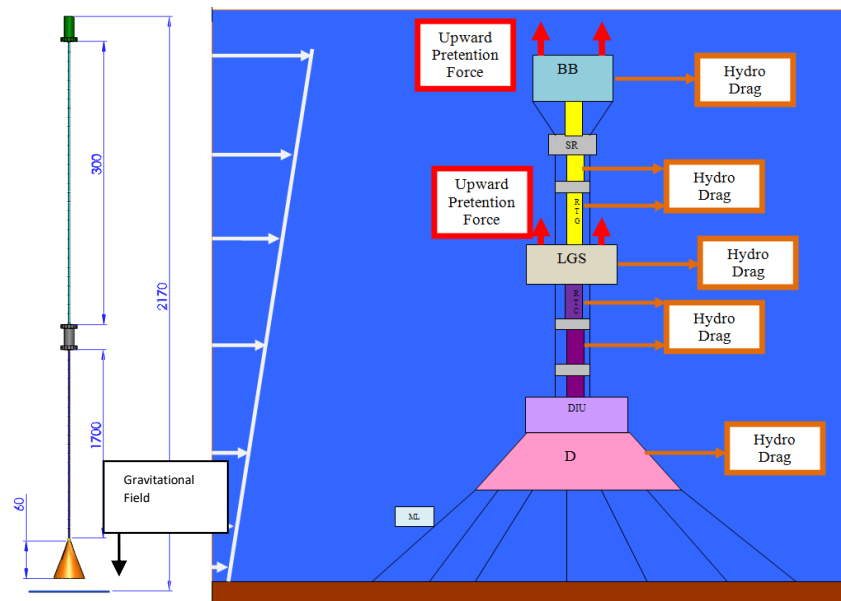
Figure 16: MIFIS Concept main dimensions for total depth 2200m from sea surface
