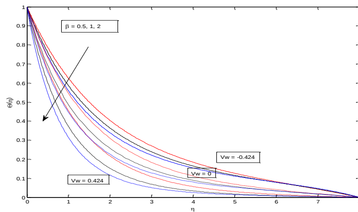
Fig.5 Temperature distribution for different values of Casson parameter \beta for various values of Suction parameter Vw with fixed values of A = 0.5 ; Pr = 0.7 ; \varepsilon = 0.2 ; R = 0.1 ; \lambda = 0.2 ; Ec = 0.1 ; Q = 0.4 ;
