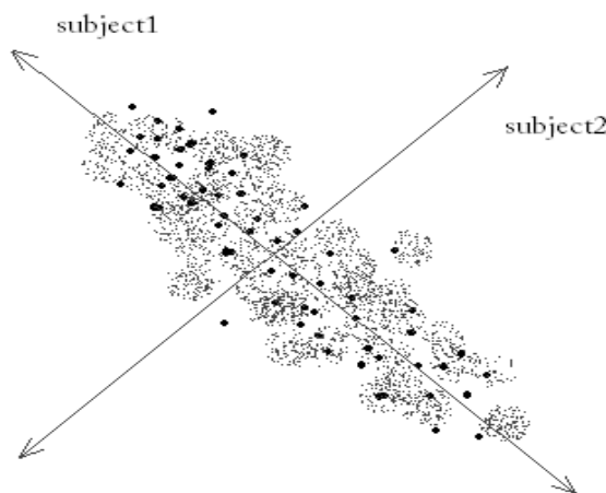
Figure: To get maximum principal component (using correlation)
