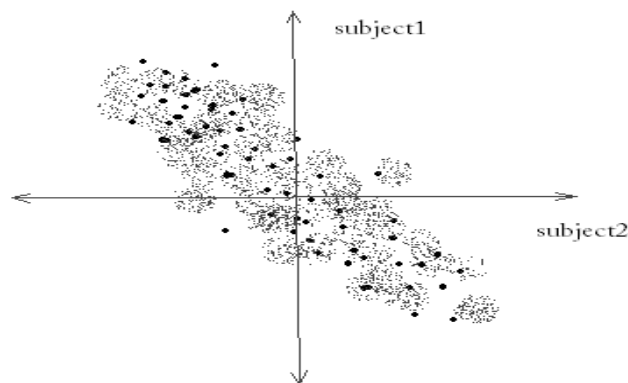
Figure: Centre mark of students in subject1 (using covariance)
