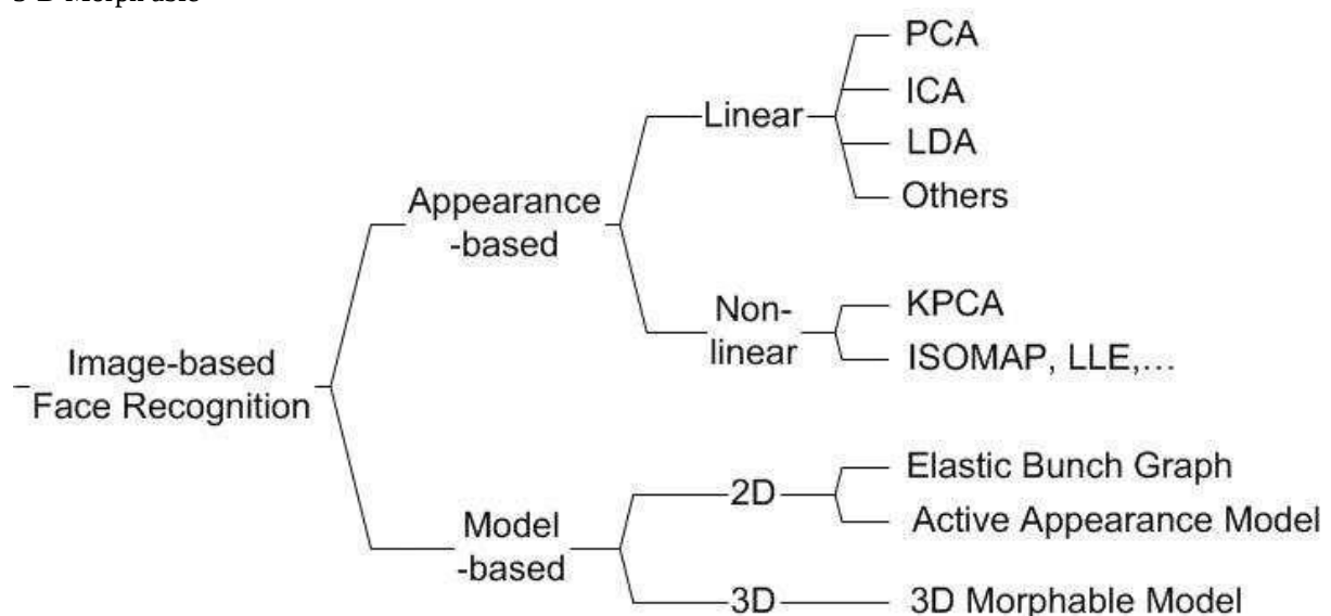
Figure shows simple classification for image-based face recognition [4]
