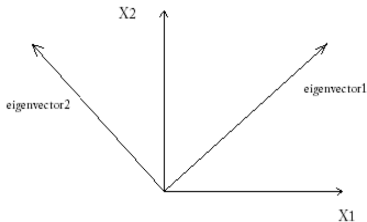
Figure: Representation of eigenvector
