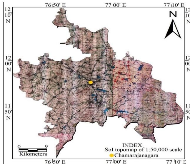
Fig.2. SoI topomap of the study area
