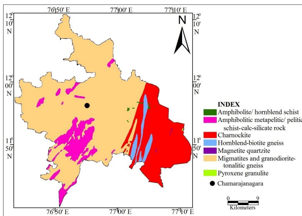
Fig.5. Lithology map of the study area
