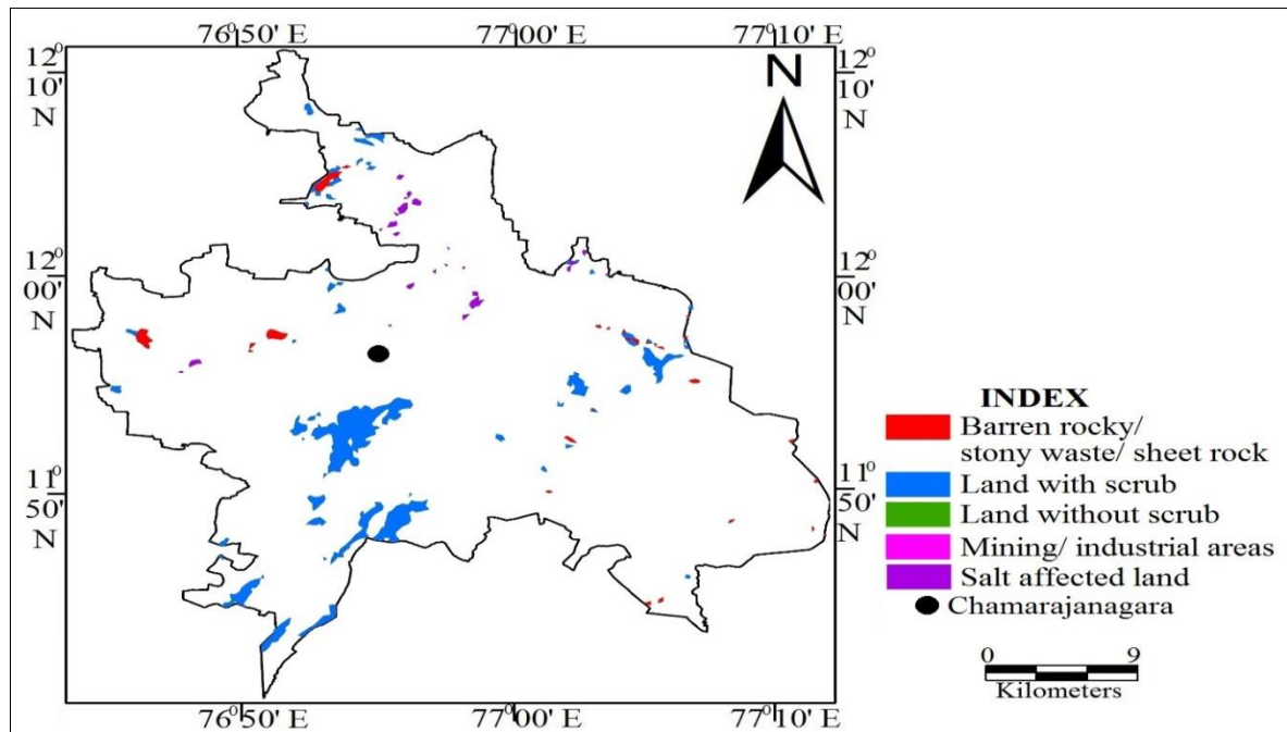
Fig.7. Wasteland categories map of the study area
