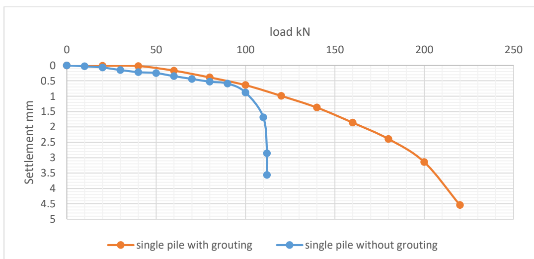
Figure (13) Relationship between static load and settlement of single pile(1/3 perforated) with and without grouting imbedded in dry medium sand
