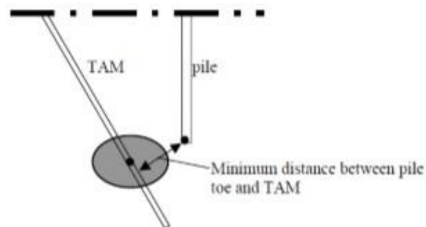
Figure (6) grouting base of piles
