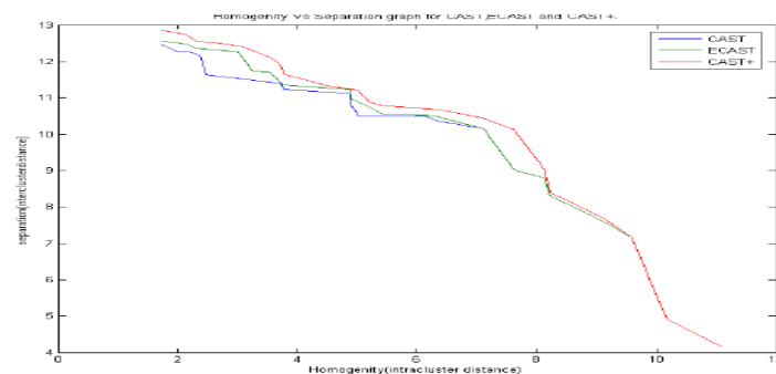
Fig 4.12 : Figure Showing the Comparison between the CAST, ECAST and proposed Algorithm .
