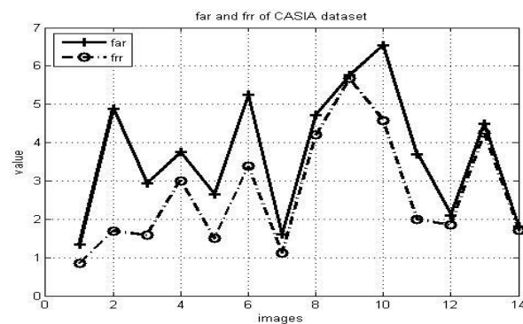
Graph1: FAR and FRR plot of CASIA v4.0 database
