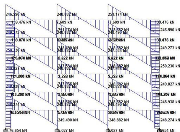
Axis shear force diag. in Y-axis
