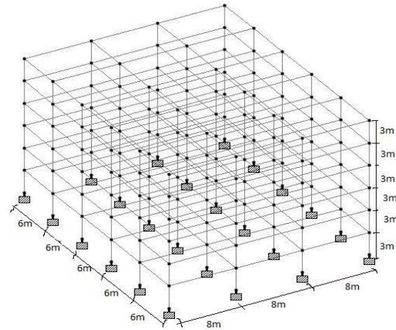
3-dimensional view of the steel building frame
