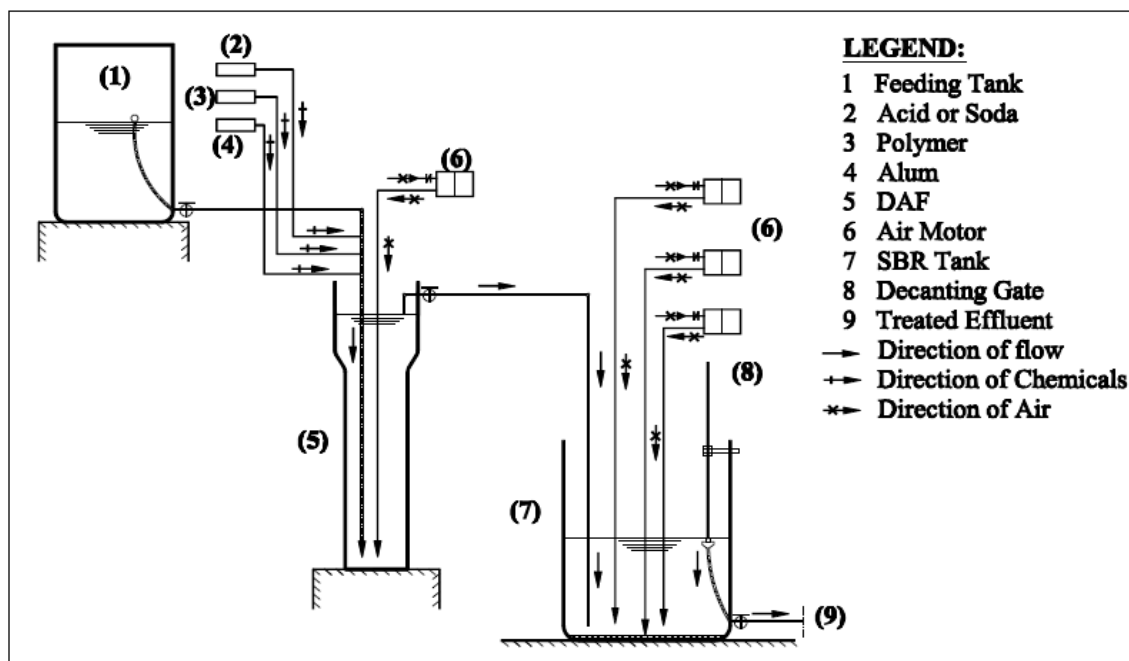
Figure (1) Flow Diagram for Pilot System
