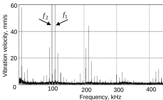
Fig. 7. Mixing frequency spectrum in an impact damage in a CFRP plate: f_1 = 111500 Hz; f_2 = 102800 Hz.
